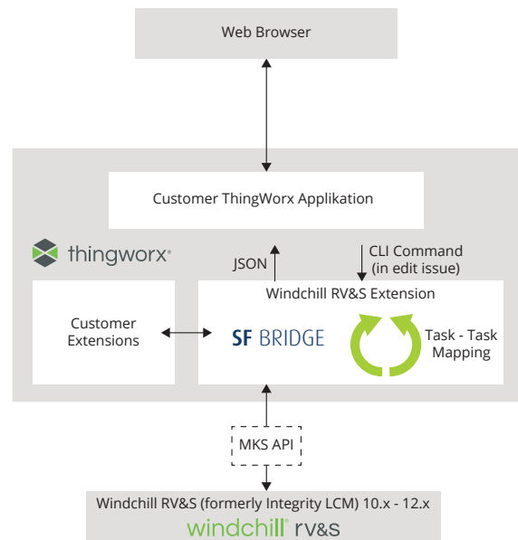
ThingWorx-Architecture with SF Bridge für PTC Windchill RV&S and ThingWorx
